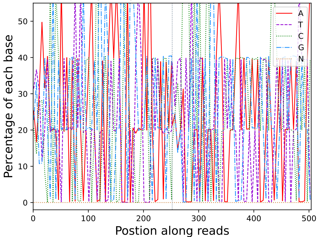
Base percentage along reads (R20111)
